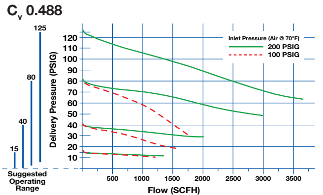
ELC4 Flow Data - EDGE Series-Liquid Cylinder
