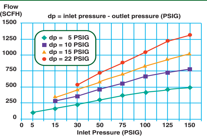
FLOW Chart - FB Series Flashback Arrestor
