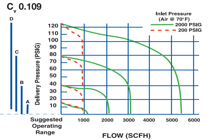
SR250 Flow Data
