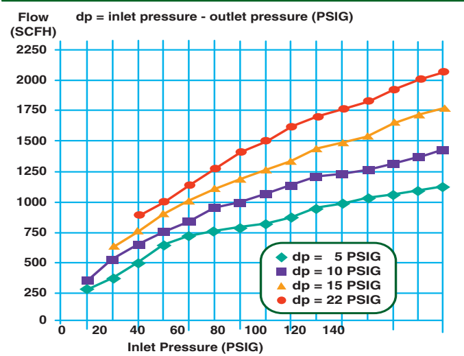
FLOW Chart - FBHC Series Flashback Arrestor
