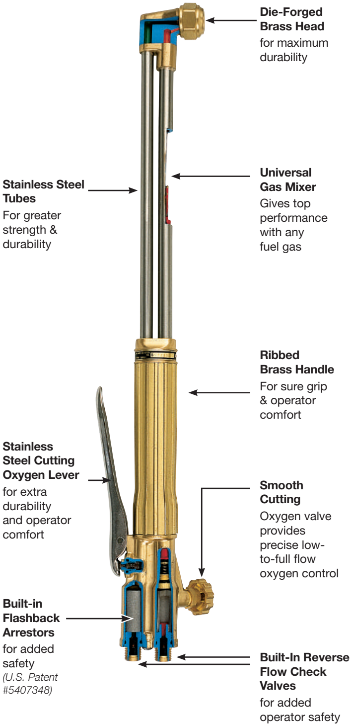
Model ST 2600FC Illustrated U.S. Patent #5407348
