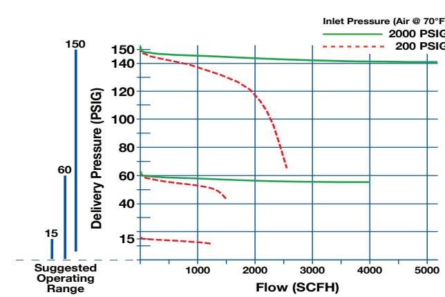
G350 Flow Data
