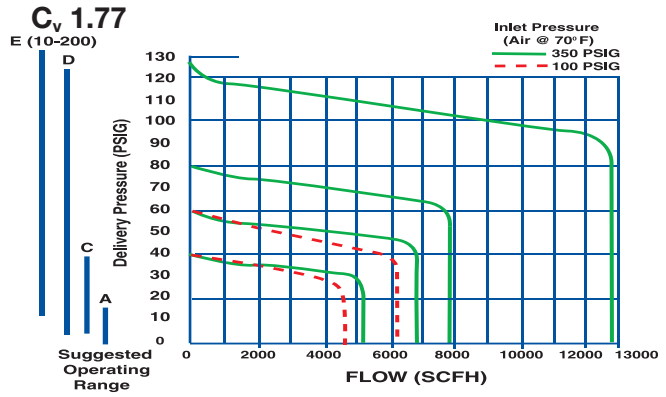
L 700 Flow Data
